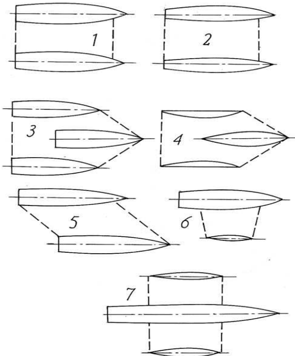
Figure 1. Studied types of multi-hulls with the traditional shape of hull: 1, 2- catamarans; 3, 4 - trimarans (as Russian terms); 5- catamaran with shifted hulls; 6- proa; 7 - ship with outriggers [2].
